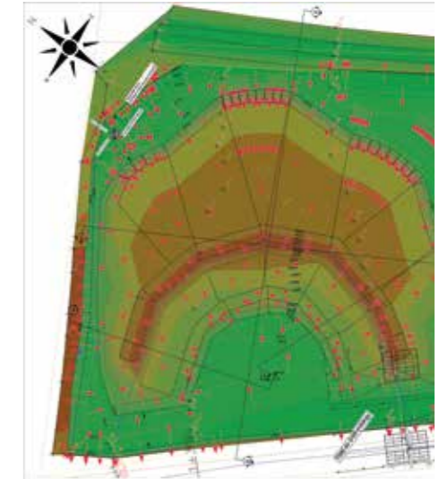
49– The inland excess water reservoir is similar to a cut-off oxbow lake in terms of both shape and river-bed geometry. Irregular shore line, asymmetric cross sections and varying lake bed depths are to be seen. The 2-metre deep graben alongside the horseshoe-shaped lake bed helps fish survive the winter. (Designer: Iván Balla, Ferenc Máriás)
